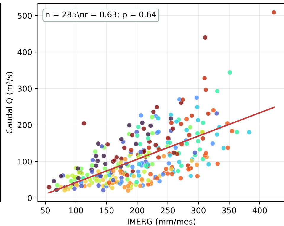
IMERG vs caudal
